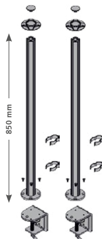
436-FP85 2 poles with clips and desk mount. Bracket, max. table top 85 mm.
