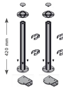
436-FP42 2 poles with clips and desk mount. Bracket, max. table top 25 mm.
